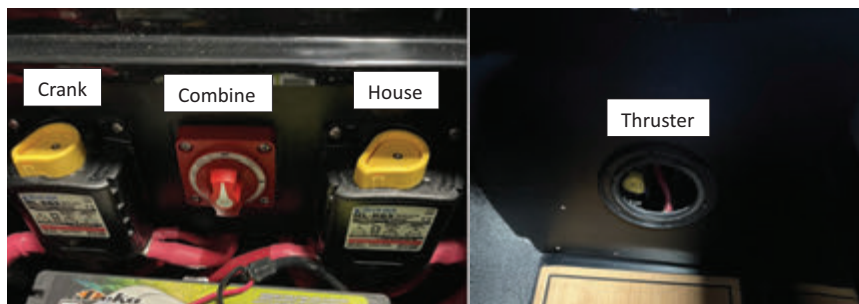
Images 1 and 2: Combine, Crank, House and Thruster Battery Locations
