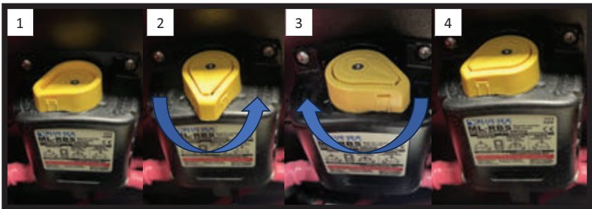
Images 8-11: Resetting a Manually Locked-On Battery Switch
